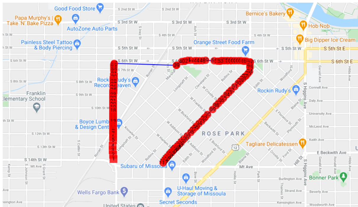
Figure 37: Plotted Data
