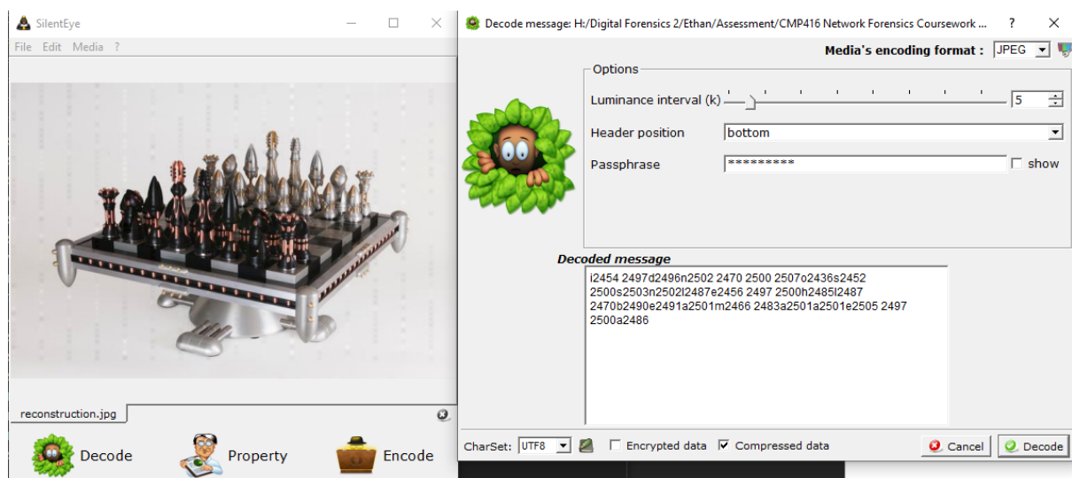
Figure 32: Decoded Steganography
