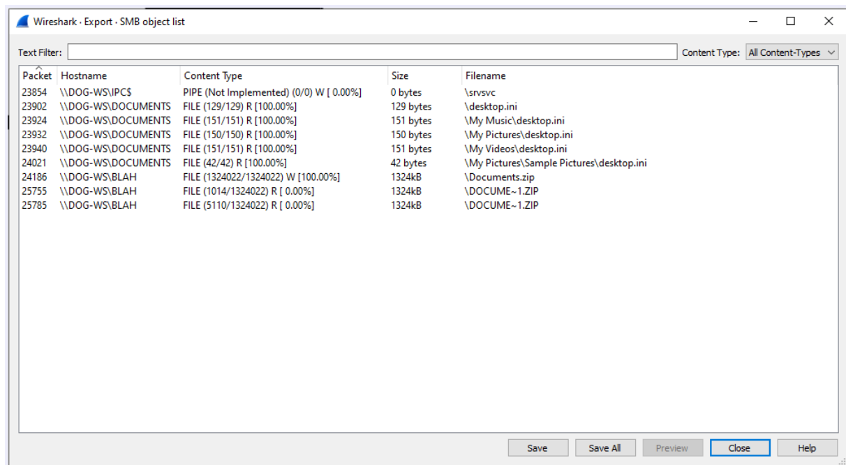
Figure 3: Exporting SMB
